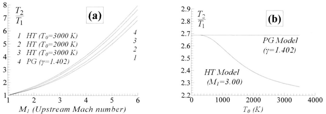
Fig. 3. Evolution of the ration T_2/T_1 (a) : versus M_1 . (b) : versus T_0 when M_1=3.00
