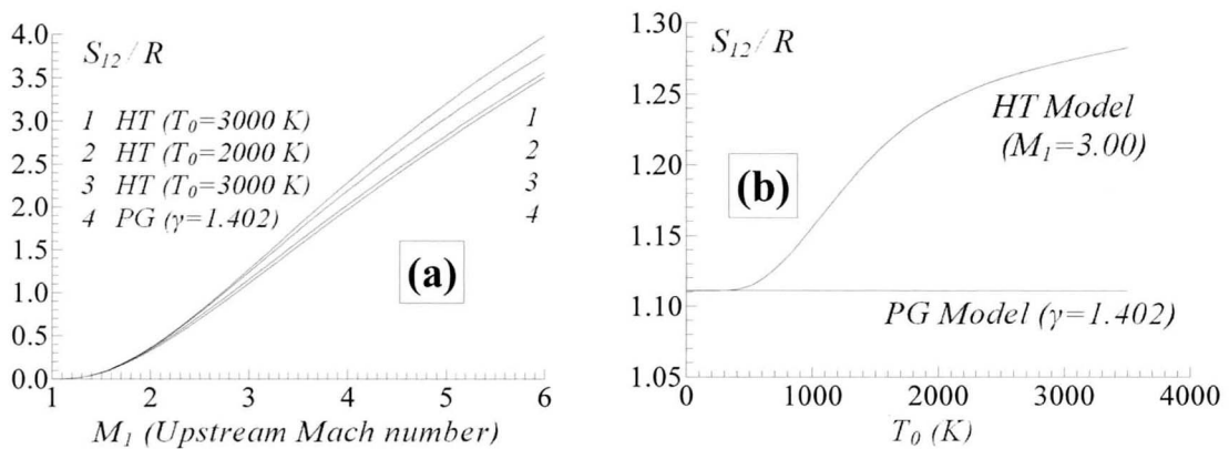
Fig. 7. Evolution of the entropy S_{12}/R (a) : versus M_1 . (b) : versus T_0 for M_1=3.00
