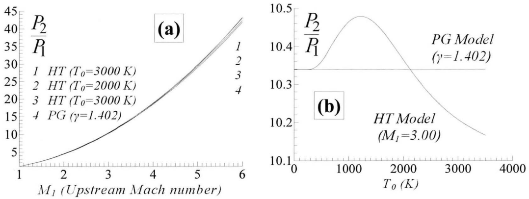
Fig. 5. Evolution of the ratio P_2/P_1 (a) : versus M_1 . (b) : versus T_0 when M_1=3.00
