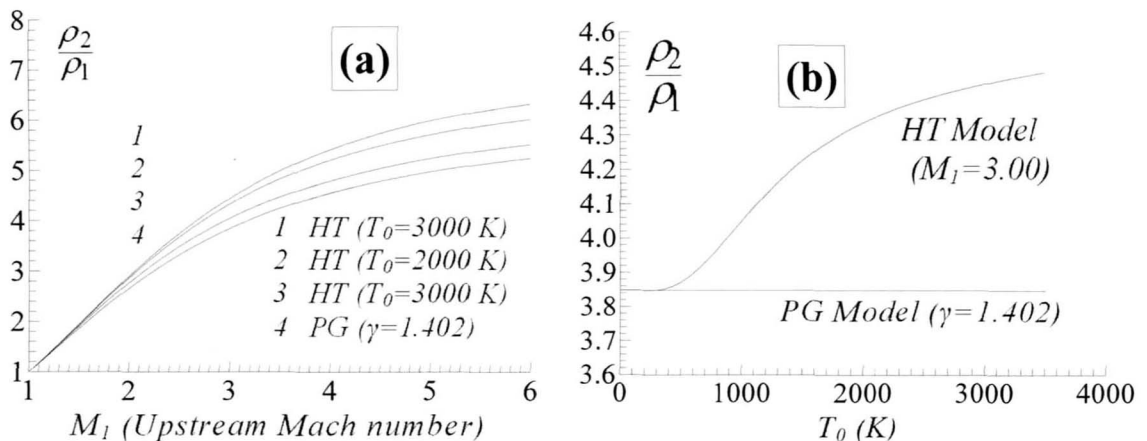
Fig. 4. Evolution of the ratio \rho_2/\rho_1 (a) : versus M_1 . (b) : versus T_0 for M_1=3.00
