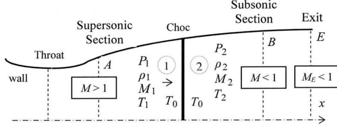
Fig. 1. Normal shock wave illustration in a nozzle
