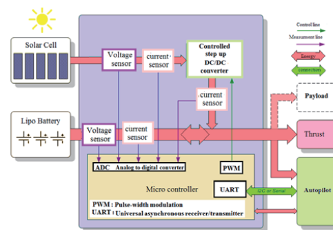
Fig. 4. Diagram used for the usage of hybrid energy in fixed wing MAVs
