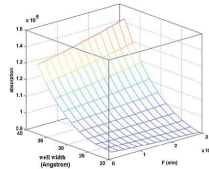
Fig. 9. Absorption coefficient on the exerted electric field and well width
