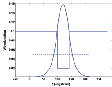
Fig. 7. Energy level and wave function acquired by solving Schrodinger equation for quantum well structure
