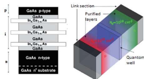
Fig. 6. A solar cell p-i-n quantum well structure
