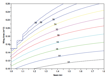
Fig. 3. Required battery capacity (Ah) for MAVs with indicated wing-span and wing area in 20 m/s cruise speed
