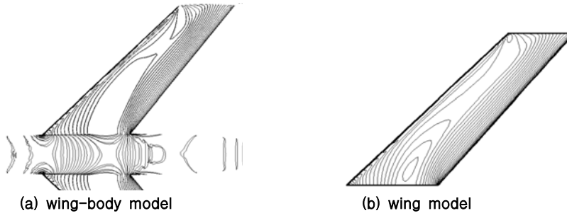
Fig. 6. Pressure coeff. contour for Mach = 0.9 and AoA = 0 degree
