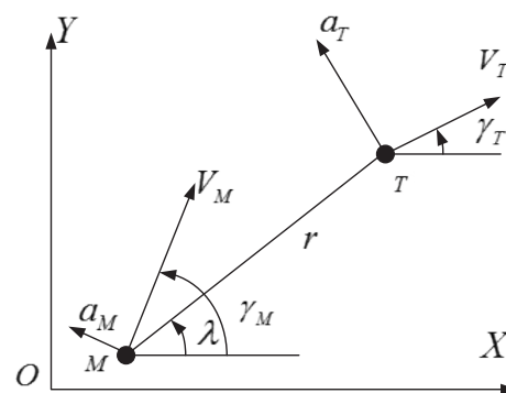
Fig. 1. Homing engagement geometry
