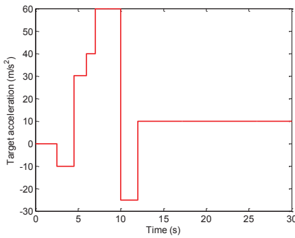
Fig. 2. Target maneuvering profile
