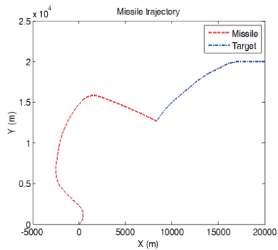
Fig. 9. Missile flight trajectory
