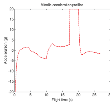
Fig. 13. Acceleration command
