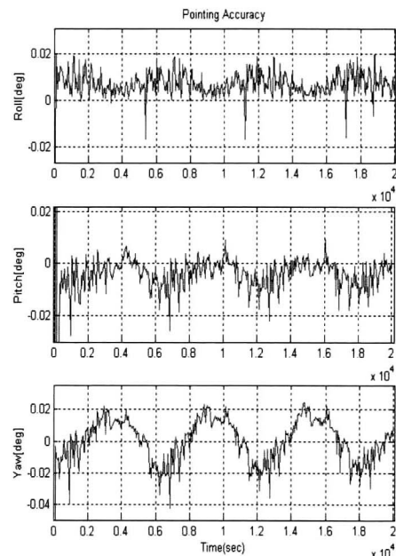
Fig. 13. Pointing Accuracy in Science Fine Submode
