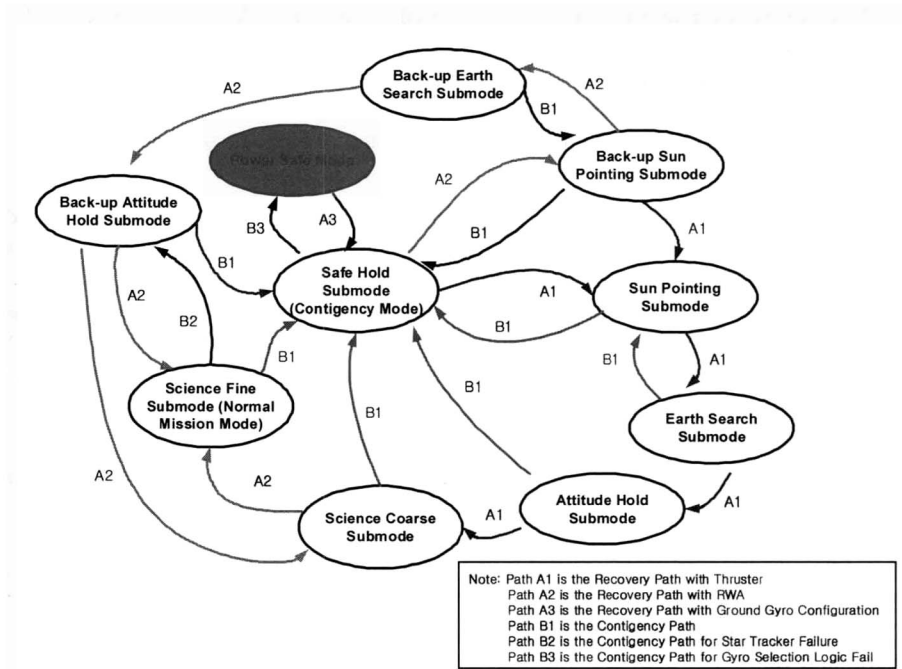
Fig. 5. AOCS Control Mode Transition Diagram
