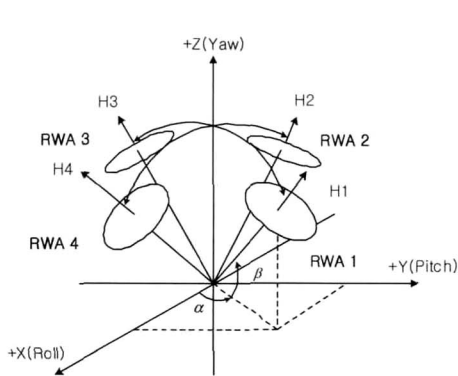
Fig. 3. Pyramid Type of Reaction Wheel Configuration
