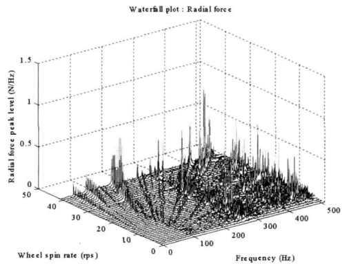
Fig. 4. Waterfall Plot of Radial Force of RWA
