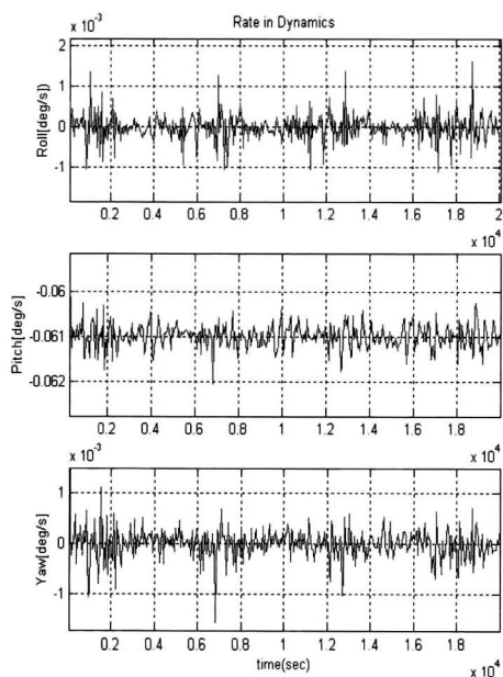
Fig. 12. Body Rate in Science Fine Submode
