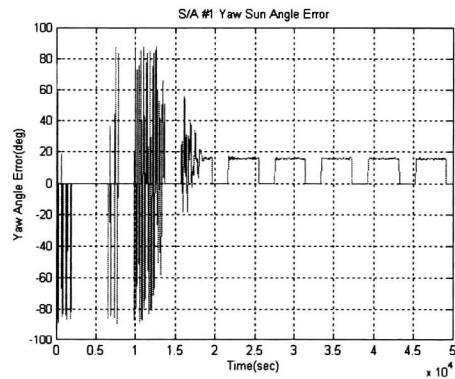
Fig. 11. Sun Angle Error in Yaw Axis
