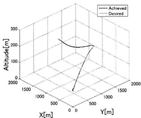
Fig. 9. Tracking performance
