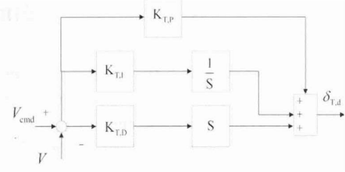
Fig. 6. PID throttle controller block diagram
