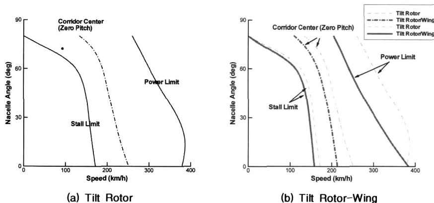
Fig. 8. Estimated Conversion Corridors of SUAV Tilt Rotor and Tilt Rotor-Wing
