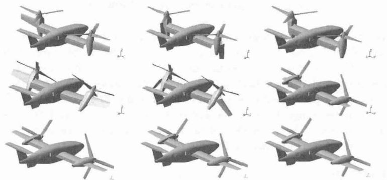
Fig. 5. Tilt Rotor-Wing Transition Concepts from Helicopter to Airplane Modes
