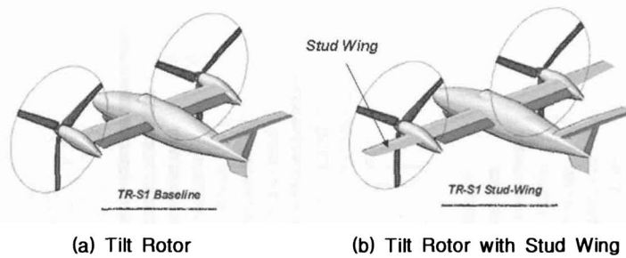
Fig. 4. Tilt Rotor-Wing Concept in Airplane Mode
