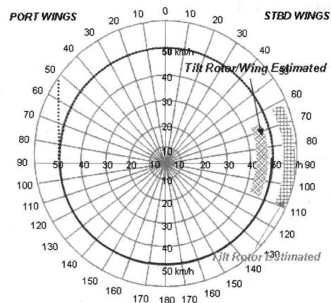
Fig. 11. Estimated Cross Wind Operational Envelope at Helicopter Landing Mode
