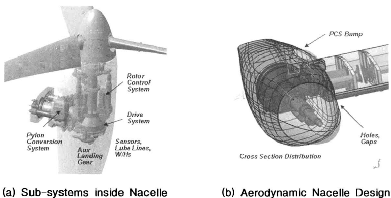
Fig. 10. Configuration Design of SUAV Wing and Nacelle
