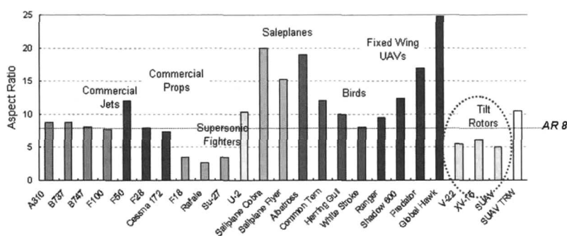
Fig. 3. Aspect Ratios of Air Vehicles
