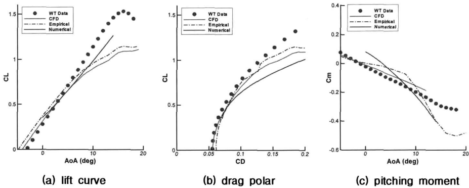
Fig. 6. Aerodynamic Characteristics of SUAV Tilt Rotor
