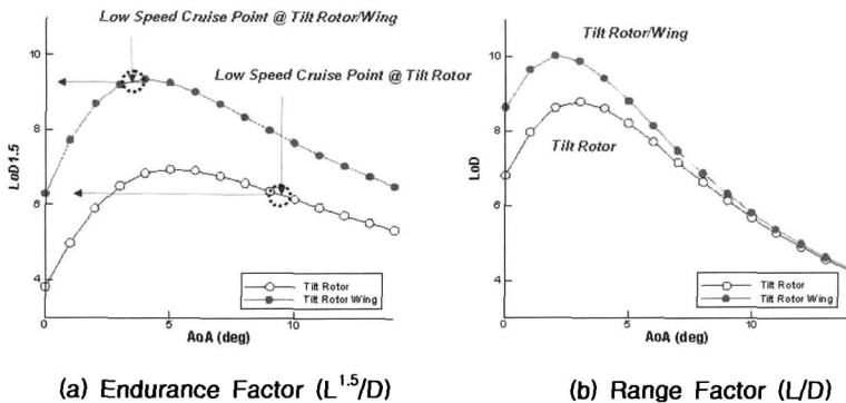
Fig. 7. Estimated Performances of SUAV Tilt Rotor and Tilt Rotor-Wing
