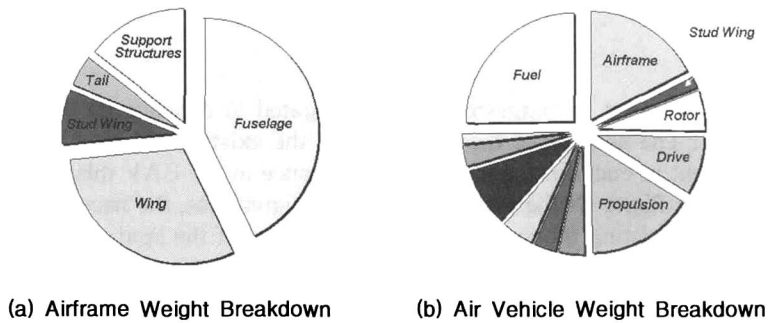
Fig. 9. Estimated Weight Breakdowns of SUAV
